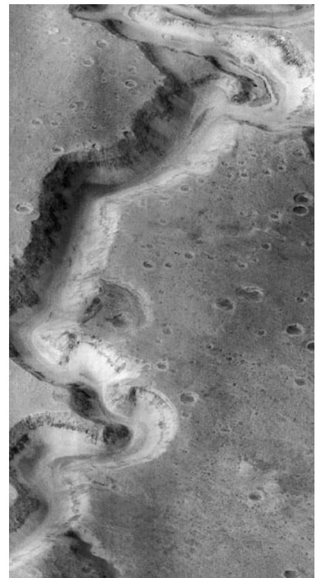
Figure 1. This image taken from the Mars Global Surveyor using the Mars Orbiter Camera reveals a 9.8 kilometer by 18.5 kilometer (6.1 mile by 11.5 mile) area of Nanedi Vallis. This feature looks very similar to a river valley on Earth, but lacks other features such as smaller channels surrounding the valley surface.
